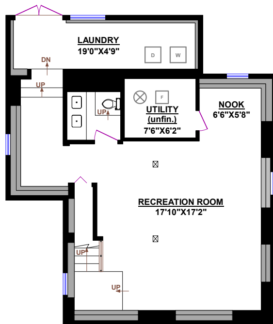
LOWER LEVEL
